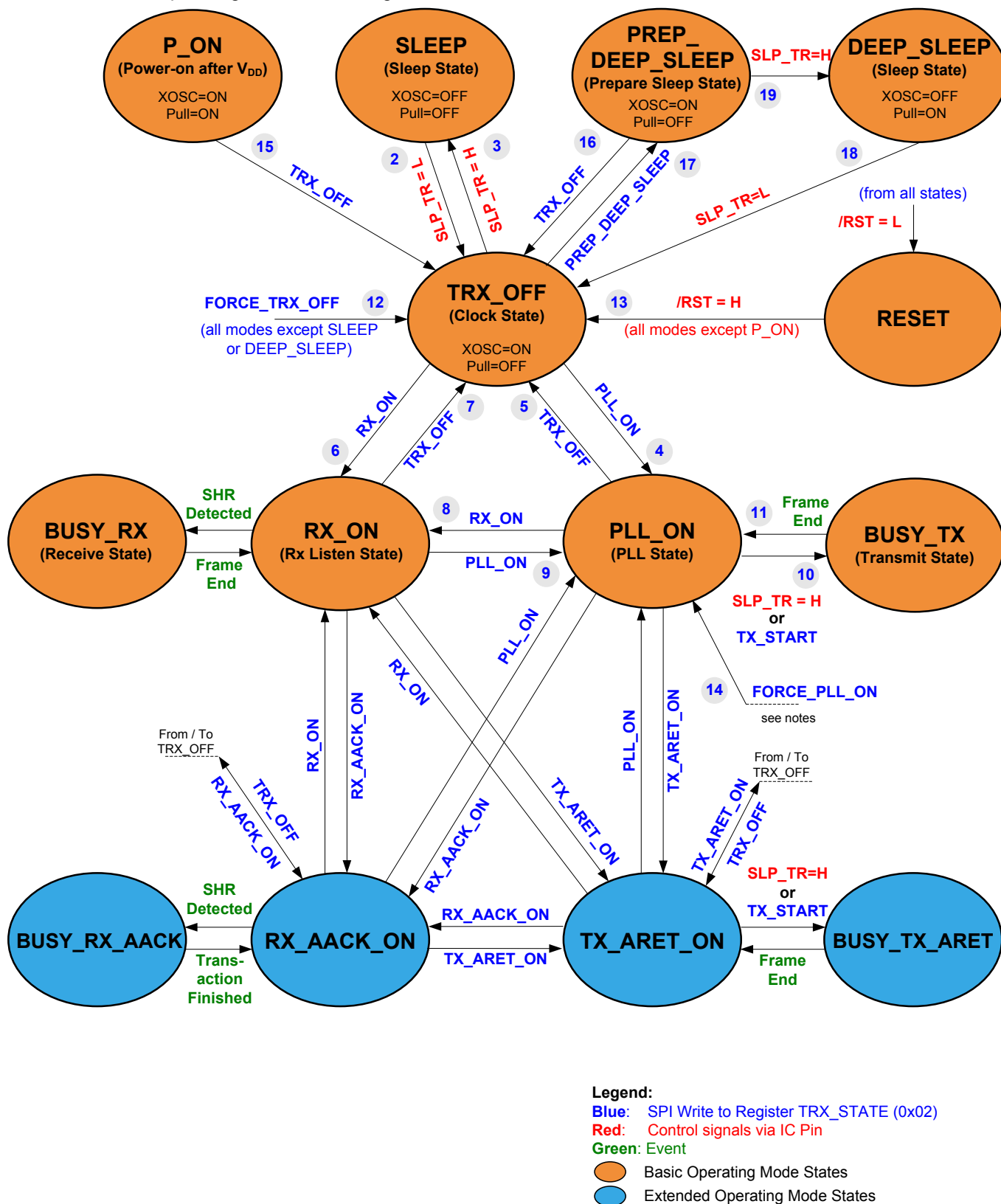
Figure 7-11. Extended Operating Mode State Diagram.
