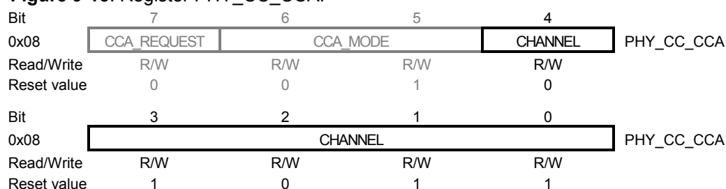
Figure 9-15. Register PHY_CC_CCA.
