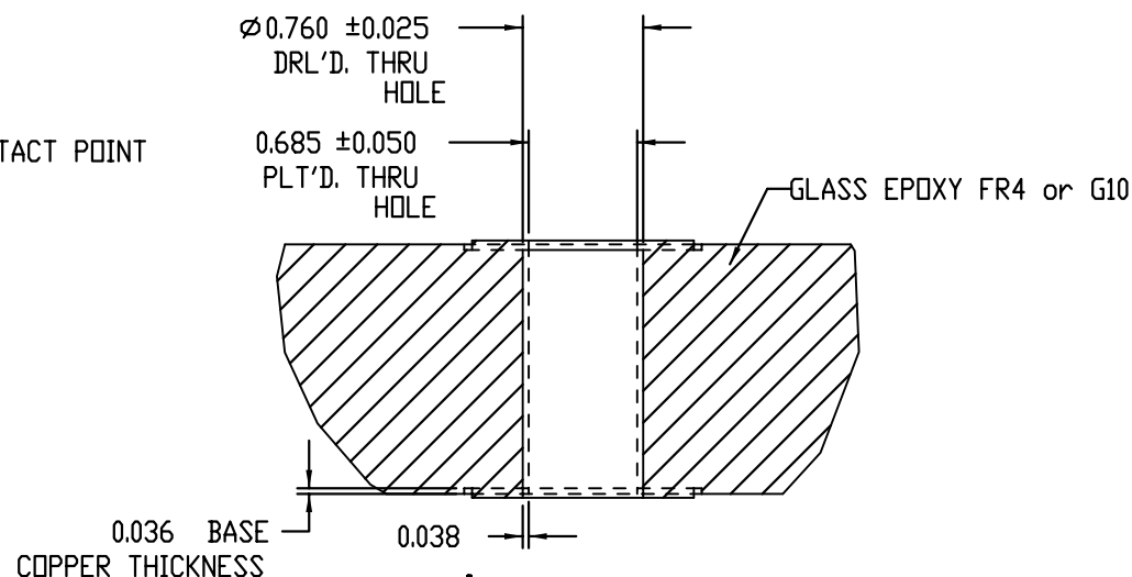
RECOMMENDED PLATED THRU HOLE DIMENSIONS FOR COMPLIANT PRESS PINS
