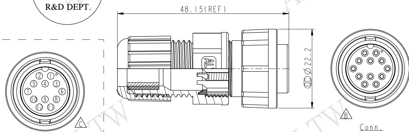
Pin Assignments Front View 前視圖
