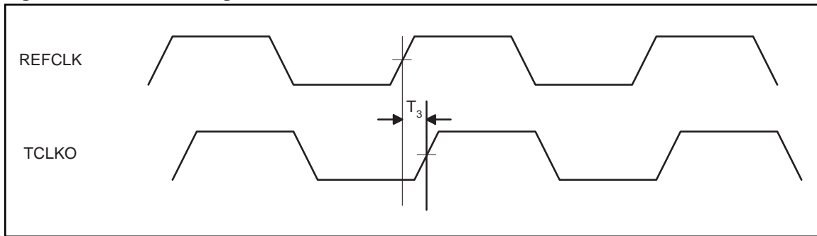
Figure 12. TCLKO Timing
