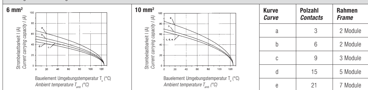
Derating Kurven / Derating curves
