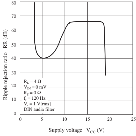
RR — V_{CC}
