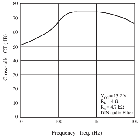
CT — freq.
