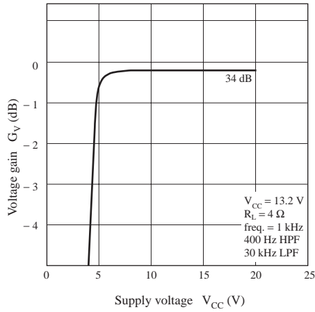
G_V - V_{CC}
