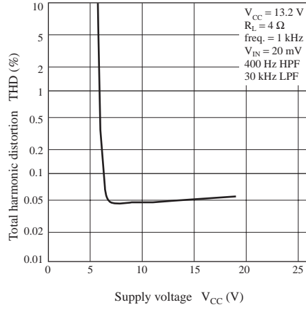
THD — V_{CC}
