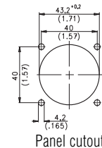
Panel cutout
