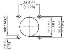
Panel cutout
