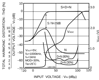
Fig.7 AM input / output characteristics
