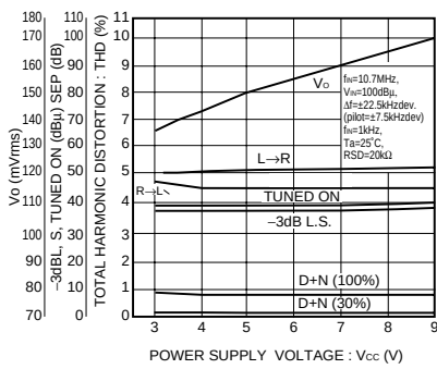
Fig.4 FM characteristics vs. power supply voltage
