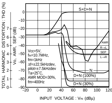
Fig.3 FM input / output characteristics
