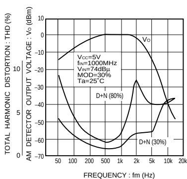
Fig.9 AM detector output and THD vs. frequency
