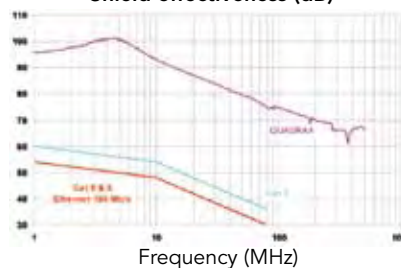
Shield effectiveness (dB)
