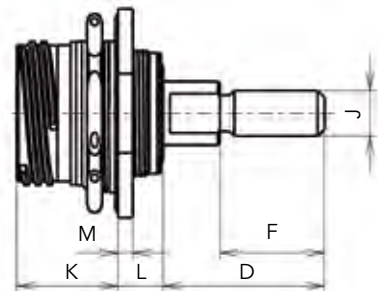
With 8D7 (jam nut receptacle)
