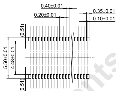
Recommended metal mask pattern Metal mask thickness: Here, 120 μm (Opening area ratio: 50%)
