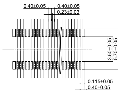
Recommended metal mask pattern Metal mask thickness: Here, 150 μm (Opening area ratio: 40%)
