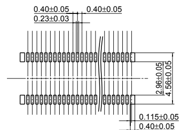
Header Recommended PC board pattern (TOP VIEW)
