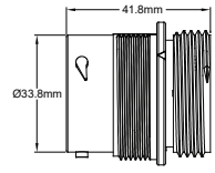
Size 18 Receptacle (WTA) Wide Thread Adapter
