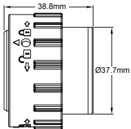
Size 24 Plug (SRA) Smooth Ring Adapter
