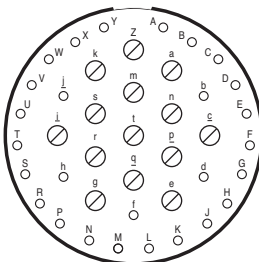
Disposition 22-41 27 contacts size 20 14 contacts size 16
