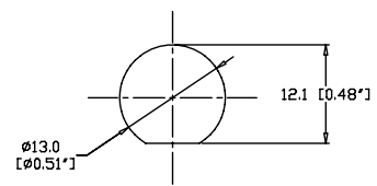
MOUNTING DETAILS
