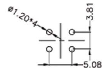
4Pin Male Connector Male Pin PCB Layout 4 Pin PCB
