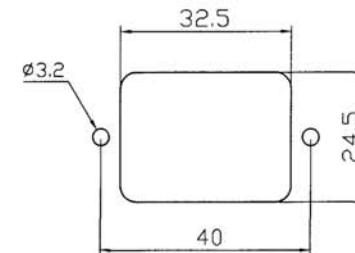
PANEL CUT-OUT
