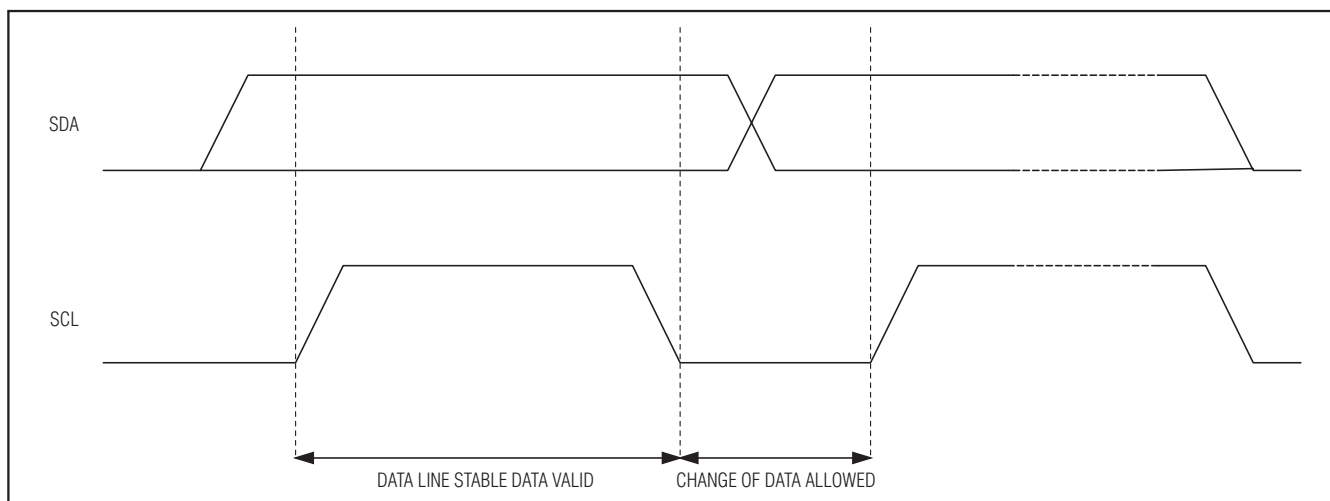
Figure 9. I 2 C Bit Transfer
