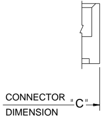
MOUNTING OPTION CODE x01 (NO MOUNTING LUGS)
