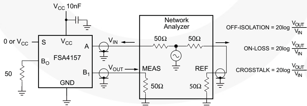
Figure 11. Off Isolation and Crosstalk
