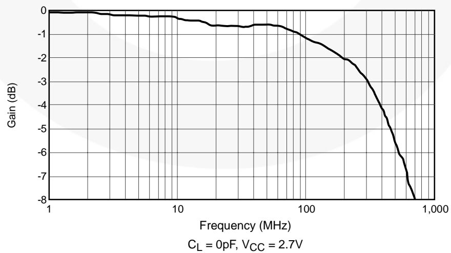
Figure 6. Bandwidth, V_{CC} = 2.7V to 5.5V
