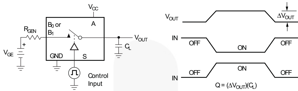
Figure 12. Charge Injection
