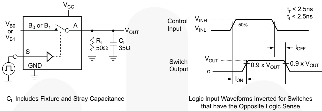
Figure 9. Turn On / Off Timing
