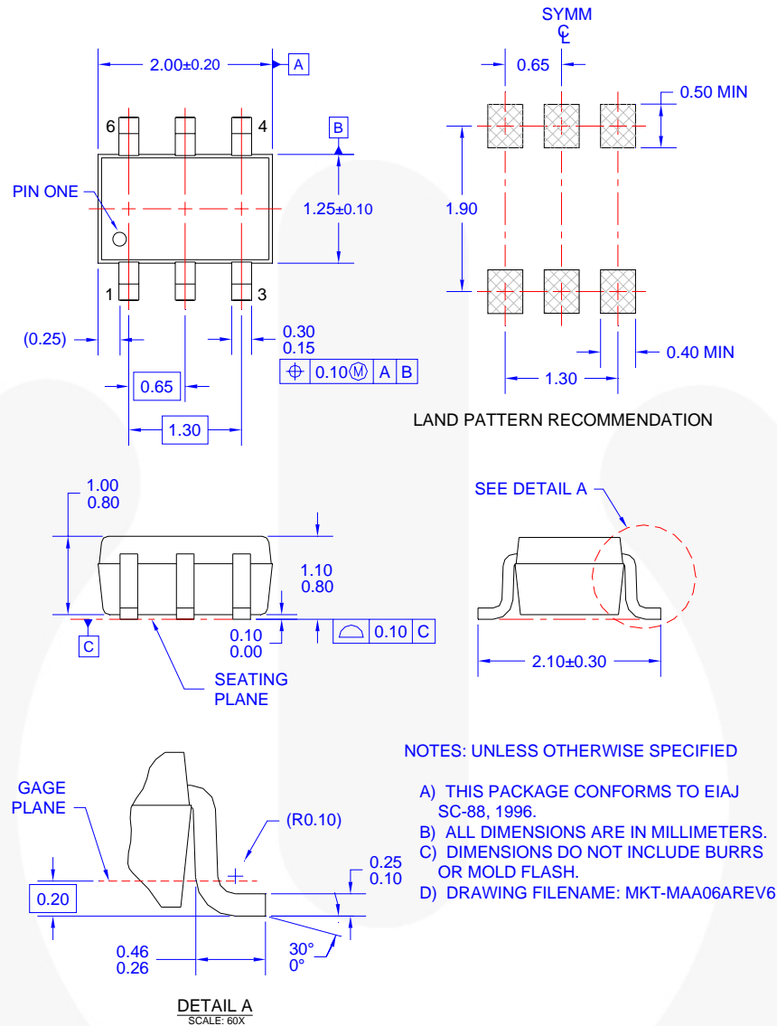
Figure 16. 6-Lead, SC70, EIAJ SC88 1.25mm Wide Package
