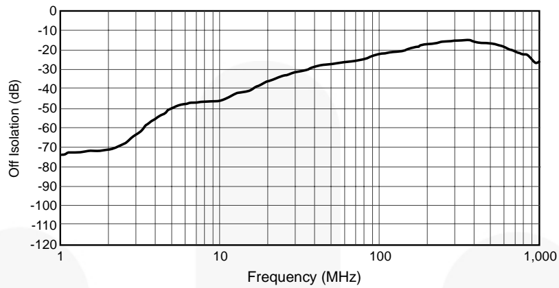
Figure 4. Off Isolation, V_{CC} = 2.7V to 5.5V
