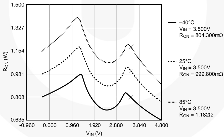
Figure 8. R_{ON} Switch On Resistance, I_{ON} = 100\text{mA} , V_{CC} = 4.5\text{V}
