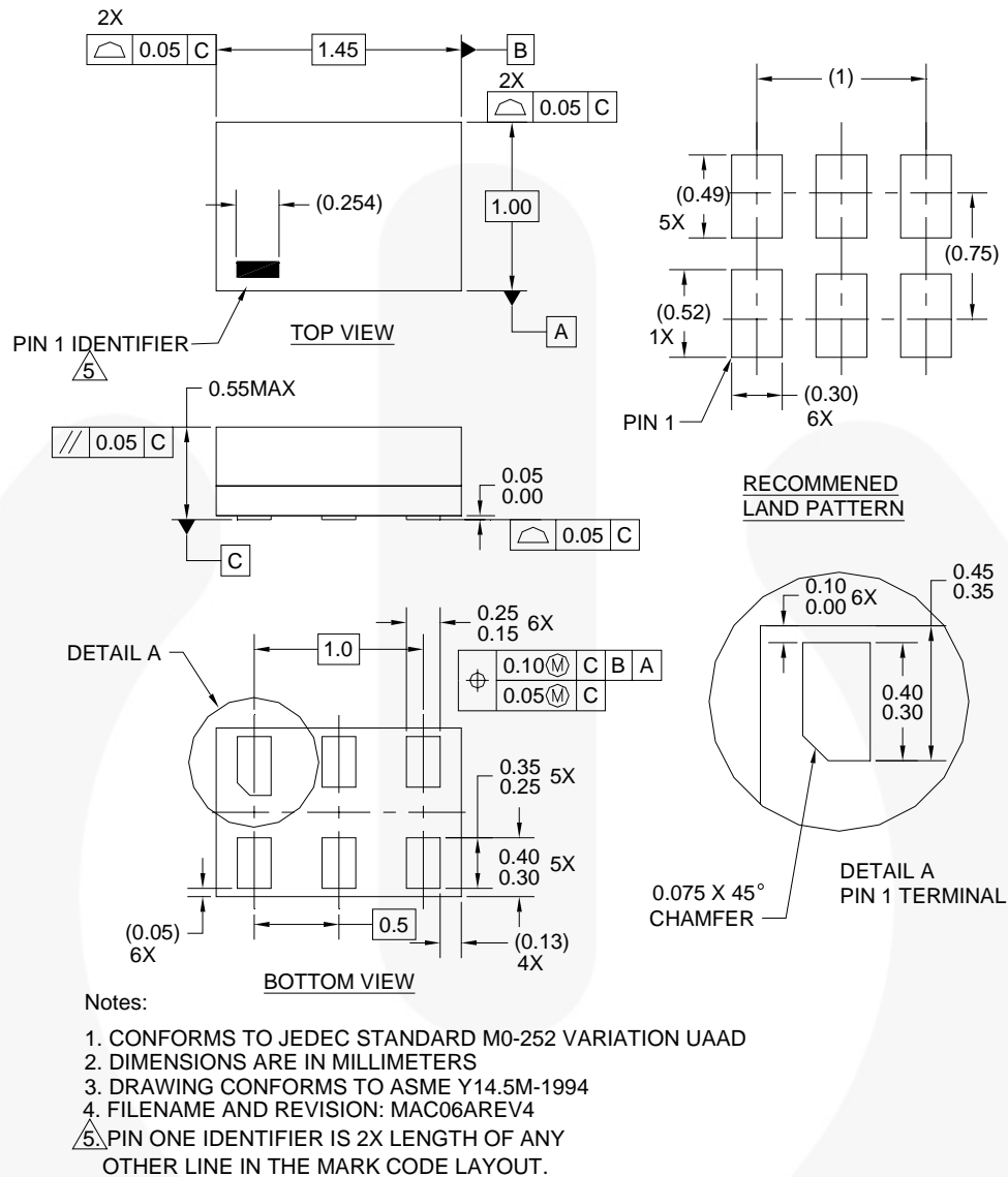
Figure 17. 6-Lead, Micropak™ 1.0mm Wide Package
