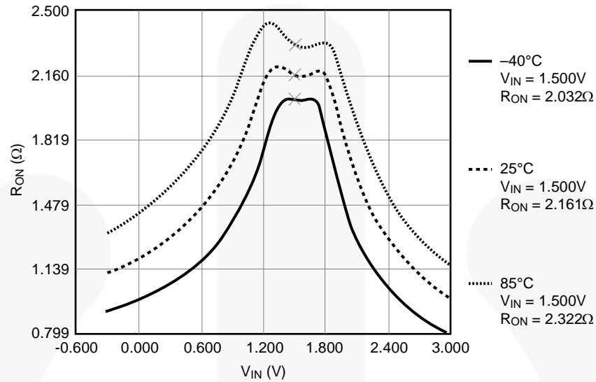
Figure 7. R_{ON} Switch On Resistance, I_{ON} = 100\text{mA} , V_{CC} = 2.7
