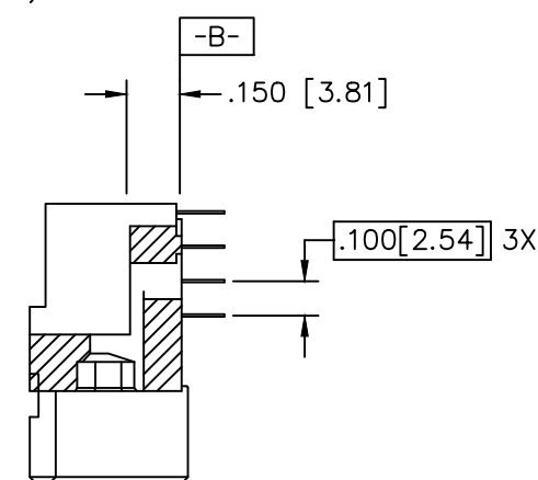
SECTION U-U
