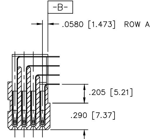
SECTION X-X
