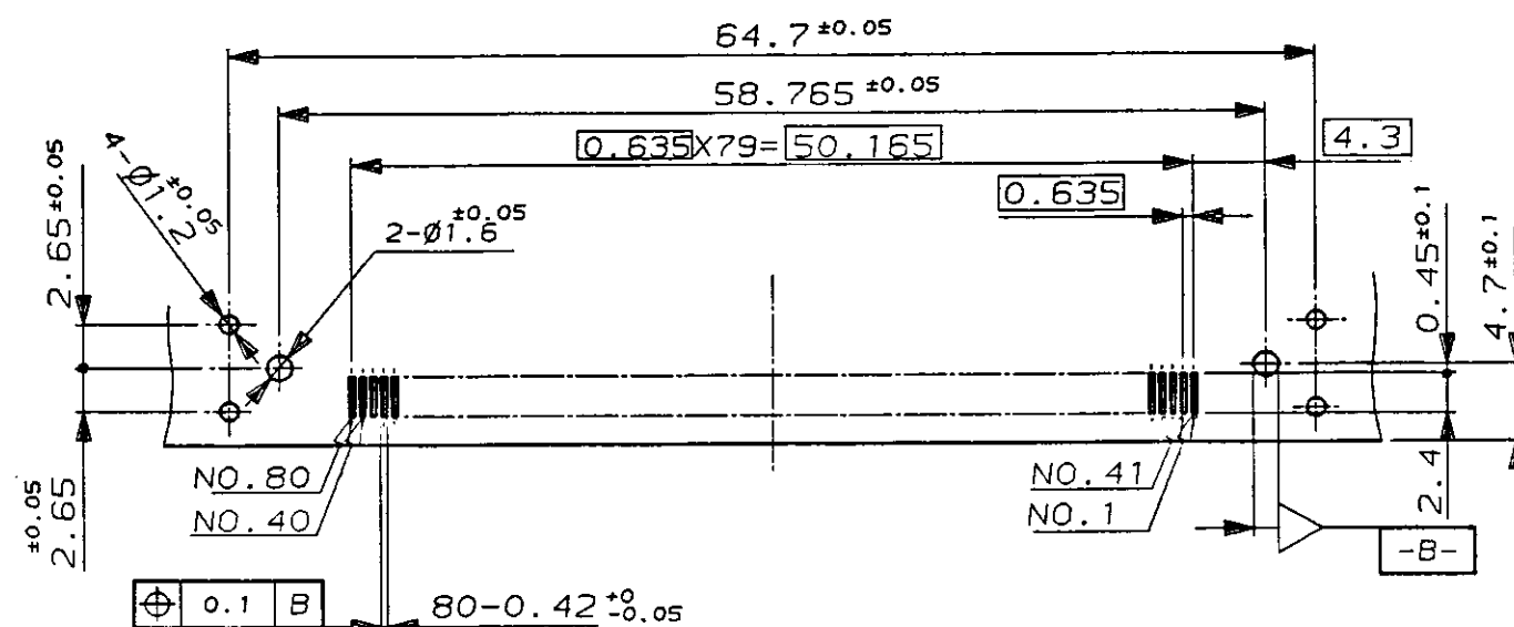
RECOMMENDED PCB LAYOUT 推奨基板取付寸法
