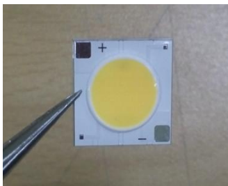
Fig.3 Proper Handling of the COB Using Tweezers
