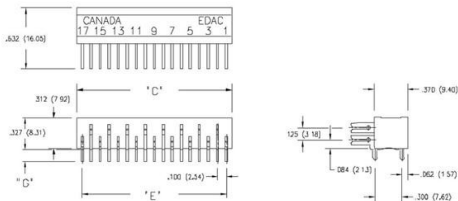
422 SERIES CONNECTOR
