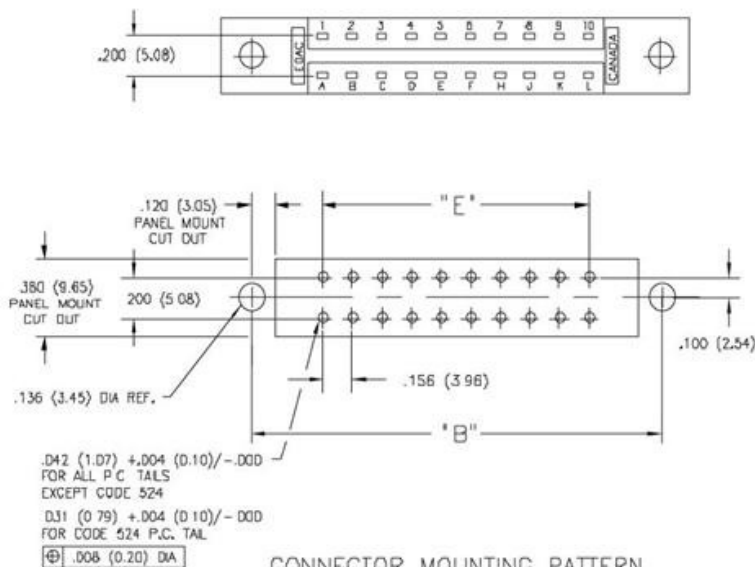
CONNECTOR MOUNTING PATTERN
