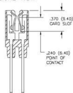
DUAL ROW
