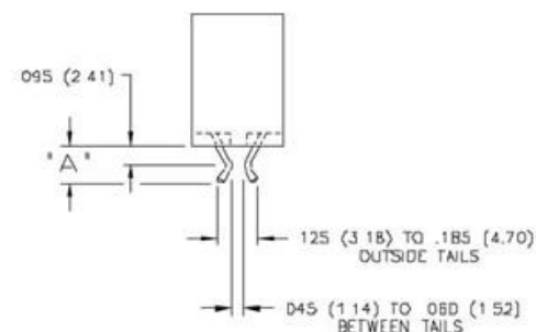
CONTACT CODE 556
