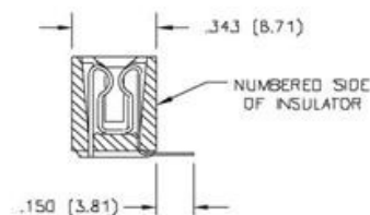
CONTACT CODE 554 BEND USES WIRE HOLE CONTACTS
