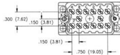
14 PIN PLUG
