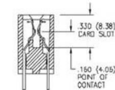
DUAL ROW
