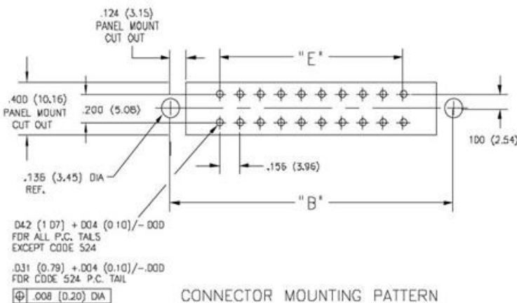
CONNECTOR MOUNTING PATTERN
