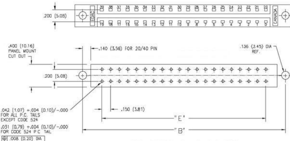
CONNECTOR MOUNTING PATTERN
