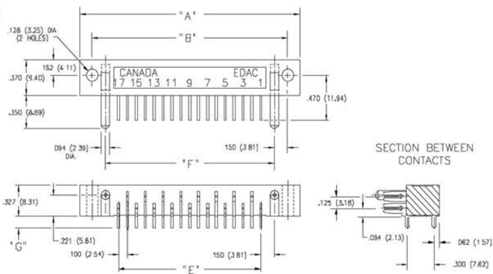
423 SERIES CONNECTOR
