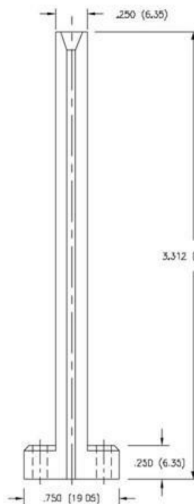
368 SERIES CARD GUIDE P/N 368-220-301
