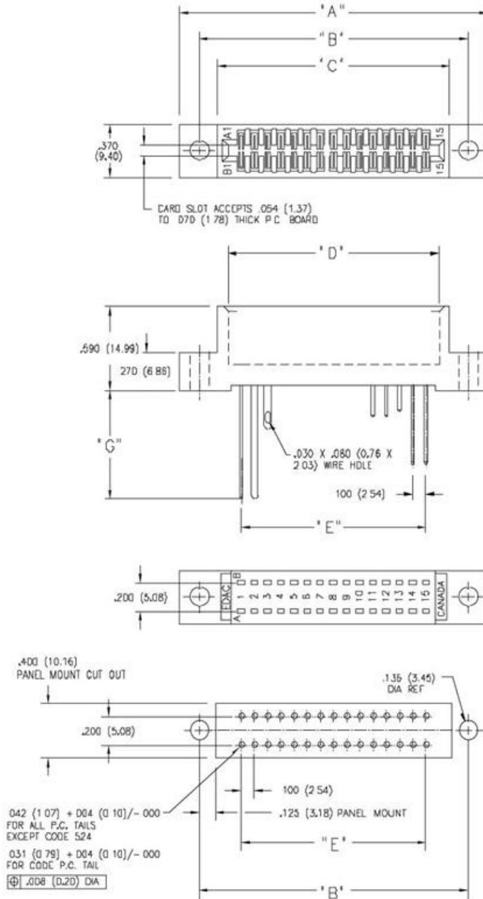
CONNECTOR MOUNTING PATTERN
