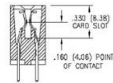
DOUBLE ROW
