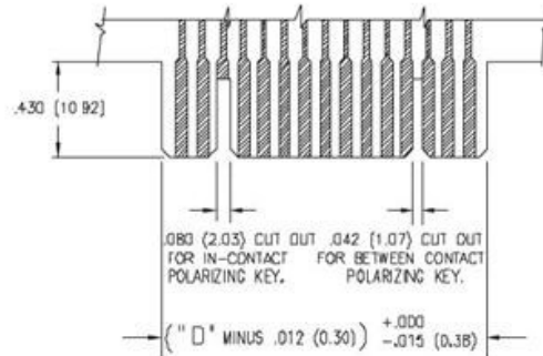
RECOMMENDED DAUGHTER BOARD
