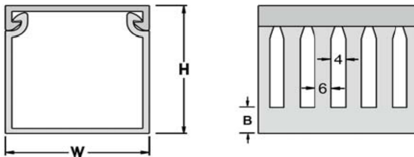
Dimensions – mm
