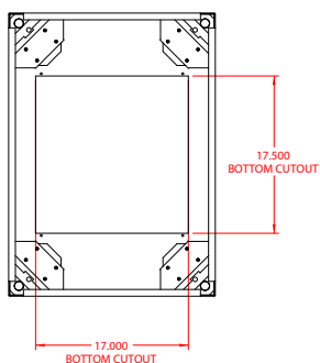
BOTTOM VIEW
