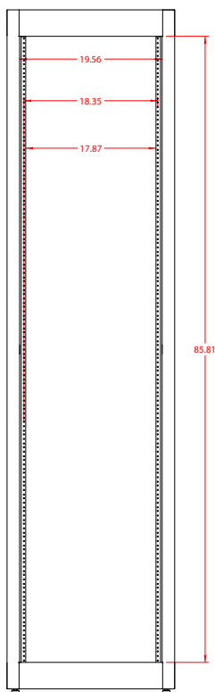
FRONT VIEW
