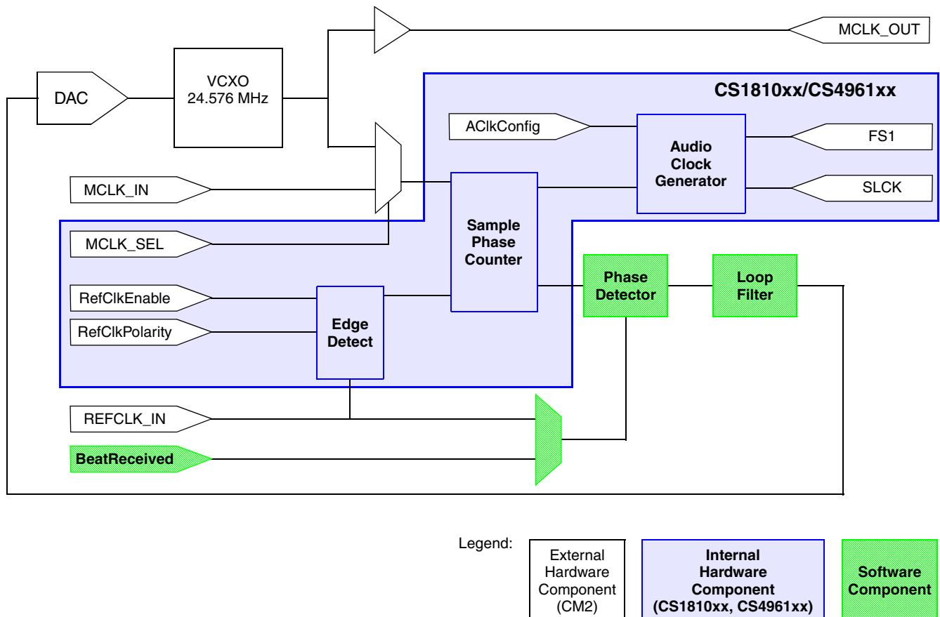
Figure 3. Audio Clock Sub-system
