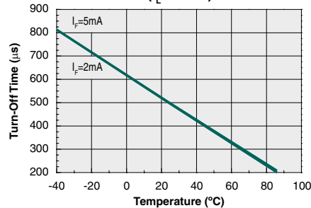
Typical Turn-Off vs. Temperature ( I_L=70\text{mA} )
