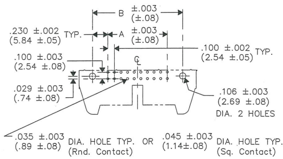
RECOMMENDED RIGHT ANGLE P.C. BOARD LAYOUT
