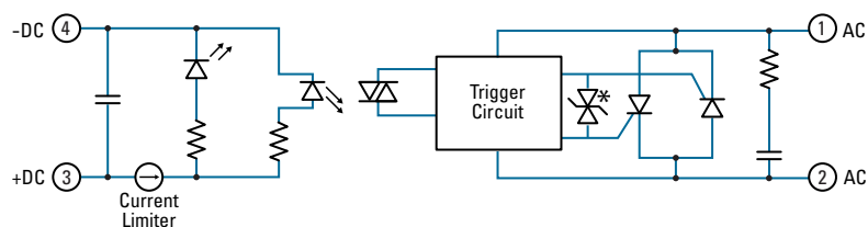
DC control
