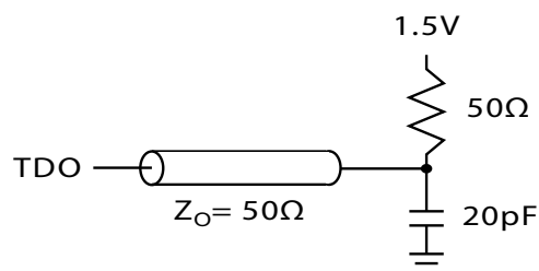
Figure 4. 3.3V TAP AC Output Load Equivalent
