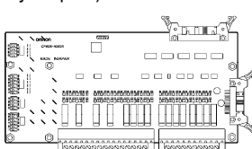
Expansion I/O board with 40 I/O points (Relay outputs)
