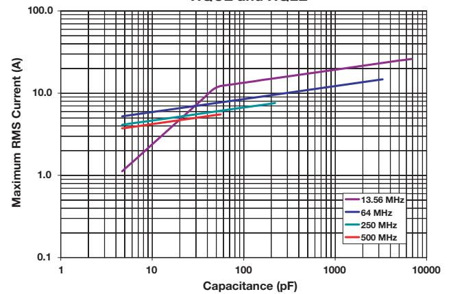
Maximum RMS Current vs. Capacitance HQCE and HQLE
