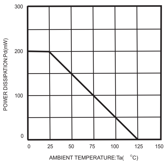
Fig.2 Derating curve
