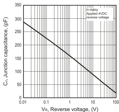
Fig.4- Junction Capacitance
