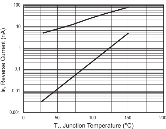
Fig.3 - Reverse Characteristics
