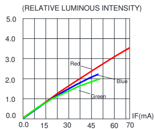
FIG.2 RELATIVE LUMINOUS INTENSITY VS. FORWARD CURRENT
