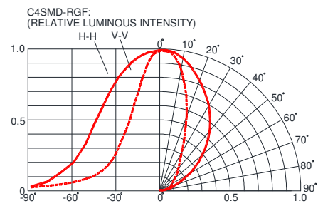
FIG.6b RED FAR FIELD PATTERN
