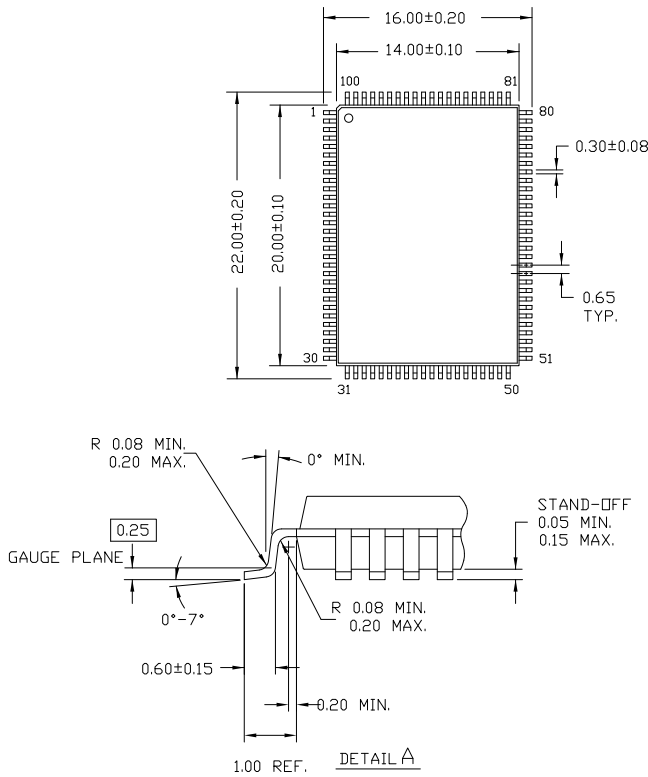
Figure 1. 100-pin TQFP (14 × 20 × 1.4 mm), 51-85050
