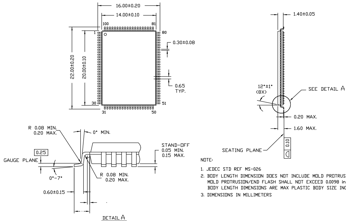
Figure 7. 100-pin TQFP (14 × 20 × 1.4 mm) A100RA Package Outline, 51-85050
