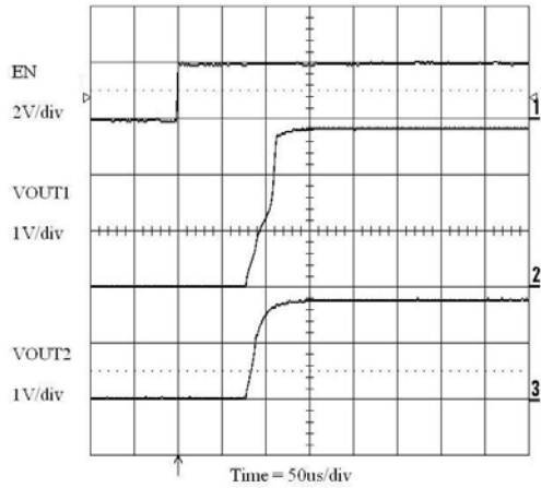
Figure 20. Enable Turn-on (300 mA/100 \mu\text{A} Loads)
