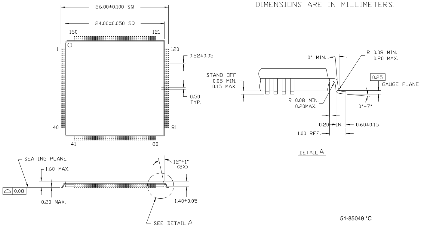
Figure 24. 160-Pin Pb-free Thin Plastic Quad Flat Pack (24 x 24 x 1.4 mm) (TQFP) A160 160 Lead Thin Plastic Quad Flatpack 24 X 24 X 1.4mm – A160
