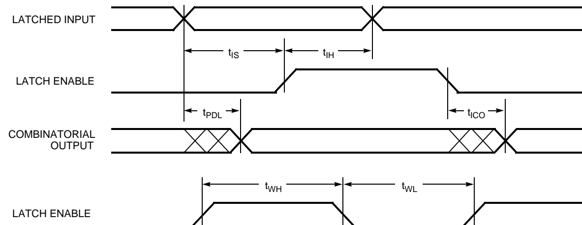
Figure 16. Latched Input
