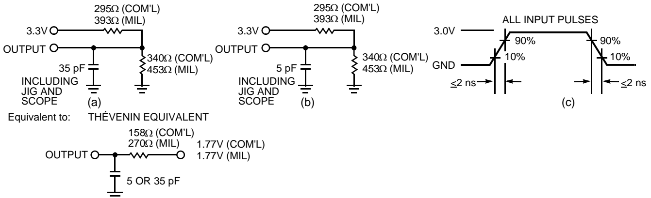
Figure 8. 3.3V AC Test Loads and Waveforms
