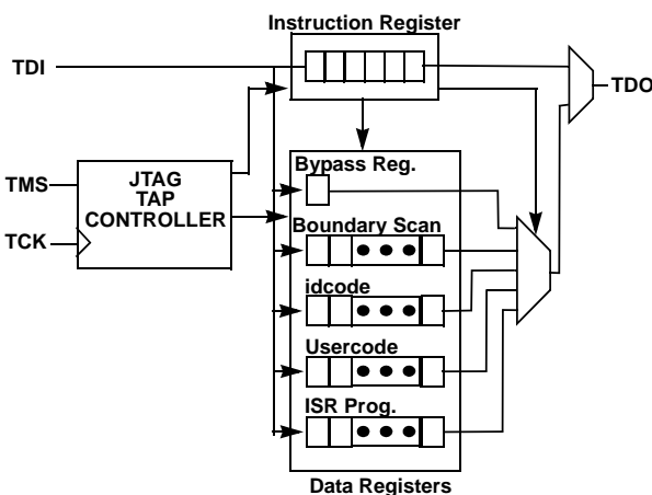
Figure 6. JTAG Interface
