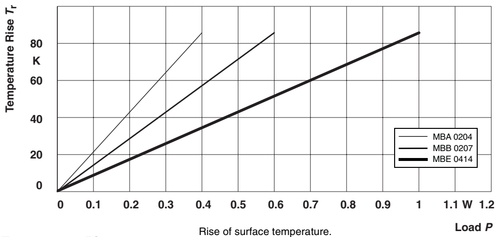
Temperature Rise
