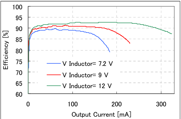
R1204xxxxxC, L=10μH (VLF302512MT-100M)
