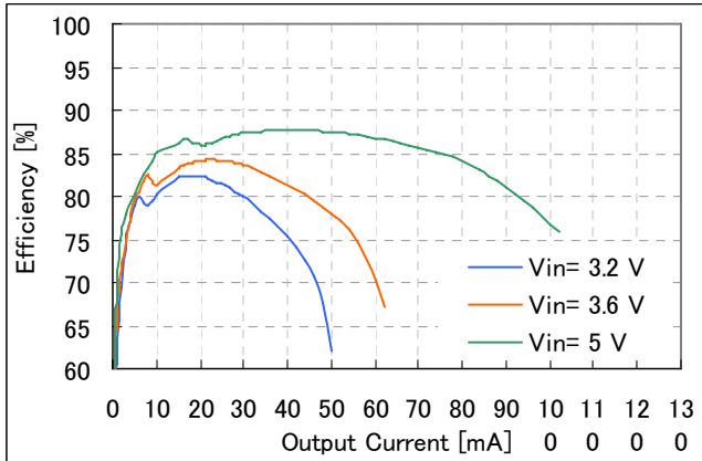
R1204xxxxxF, L=22μH (VLF302512MT-220M)
