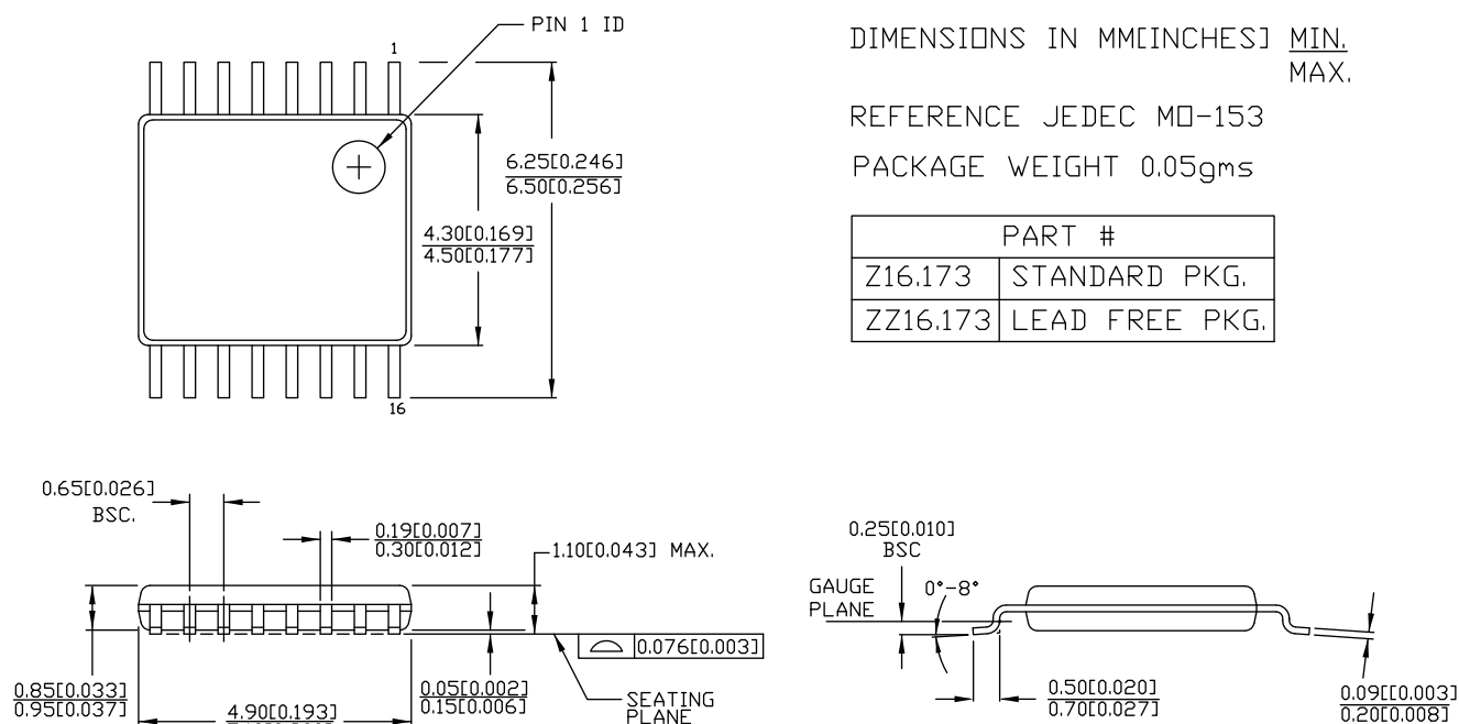
Figure 14. 16-Pin TSSOP 4.40 mm Body
