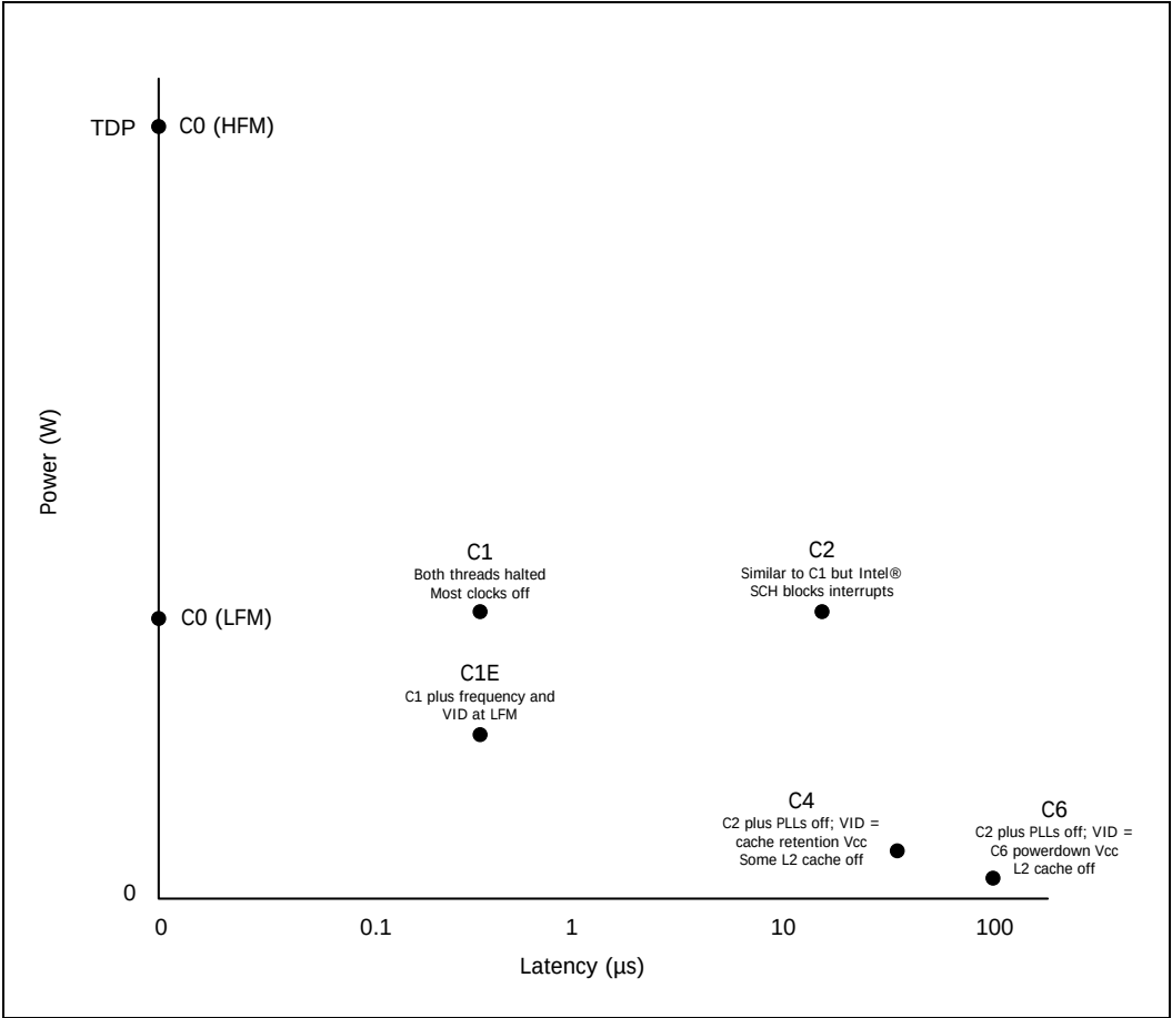
Figure 5. Exit Latency Table
