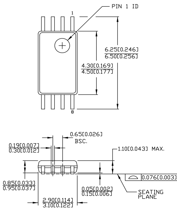
Figure 15. 8-pin (4.40-mm Body) TSSOP (Thin Shrunk Small Outline Package)
