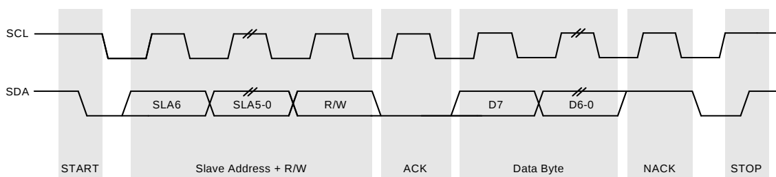
Figure 19.3. SMBus Transaction
