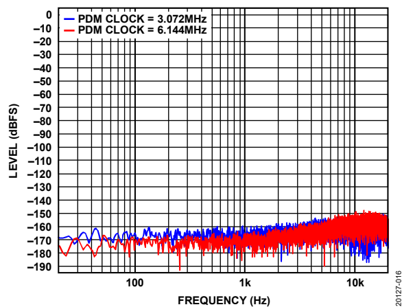
Figure 16. FFT, No Signal, f_s = 48 kHz Throughout, Signal Path = SDATAI_x to FastDSP to PDM Output
