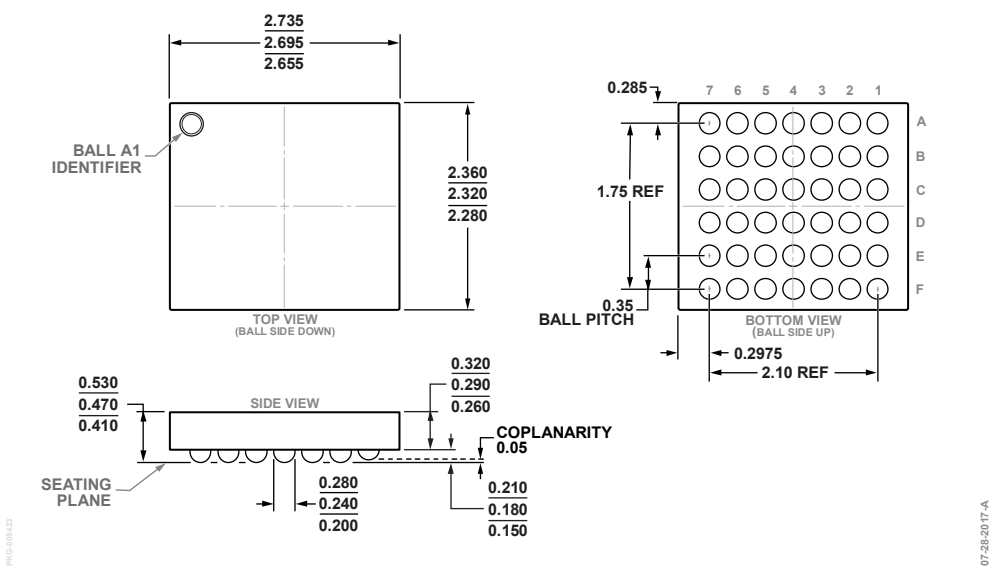
Figure 72. 42-Ball Wafer Level Chip Scale Package [WLCSP] (CB-42-2) Dimensions shown in millimeters
