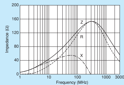
BLM31PG121SZ1/BLM31PG121SH1
