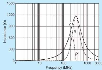
BLM18BB331SZ1/BLM18BB331SH1
