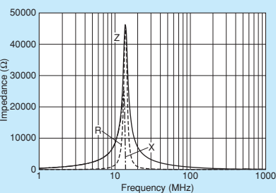
NFZ32BW451HZ10
