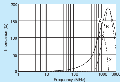
BLM18BA100SZ1/BLM18BA100SH1
