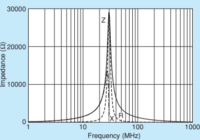
NFZ32BW151HZ10
