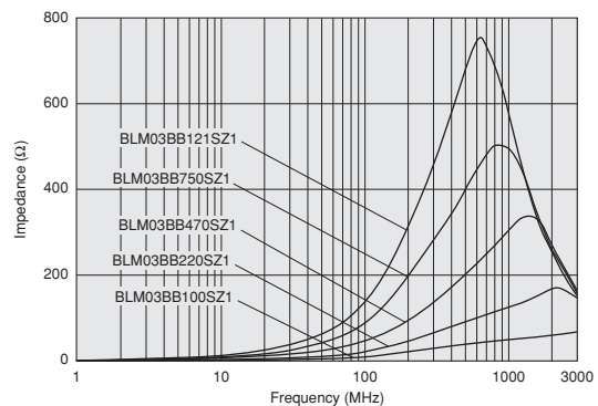
BLM03BB Series
