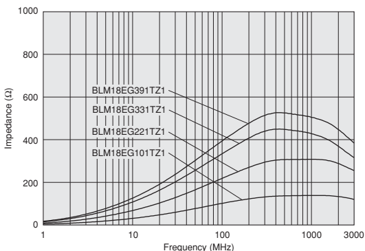
BLM18EG_TZ1 Series
