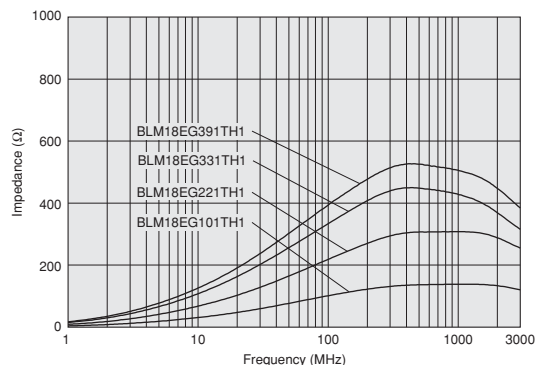
BLM18EG_TH1 Series
