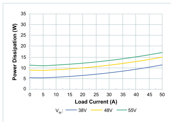
Figure 5 — Power dissipation at T_{CASE} = -40^{\circ}\text{C}
