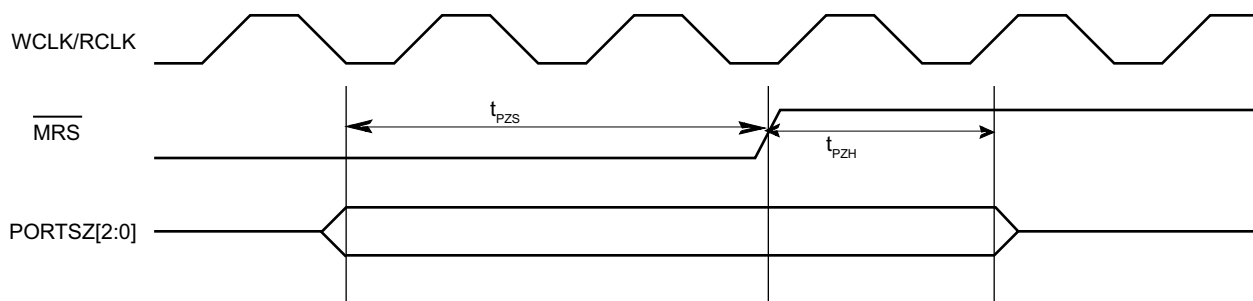
Figure 9. MRS to PORTSZ[2:0]
