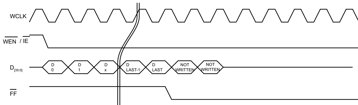
Figure 18. Full Flag Assertion
