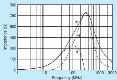
BLM15BX471SZ1
