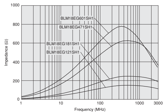
BLM18EG_SH1 Series
