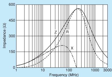
BLM18PG471SZ1/BLM18PG471SH1
