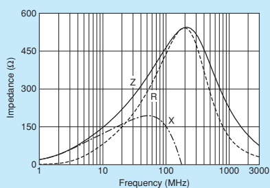
BLM18AG471SZ1/BLM18AG471SH1
