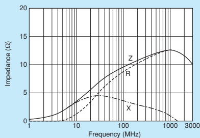
BLM03AG100SZ1
