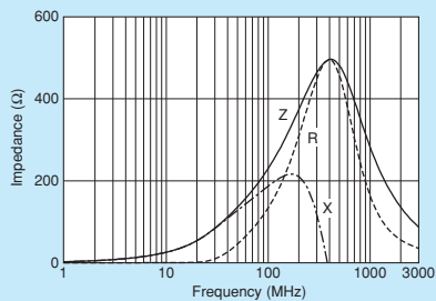
BLM18BD221SZ1/BLM18BD221SH1
