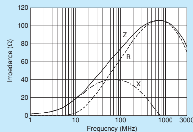
BLM15AX700SZ1
