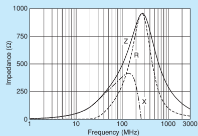
BLM18BD152SZ1/BLM18BD152SH1
