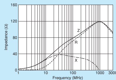
BLM03AG800SZ1
