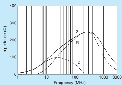
BLM18SG221TZ1
