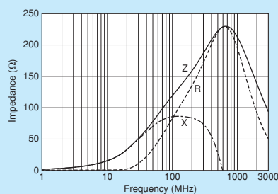
BLM15BX121SZ1
