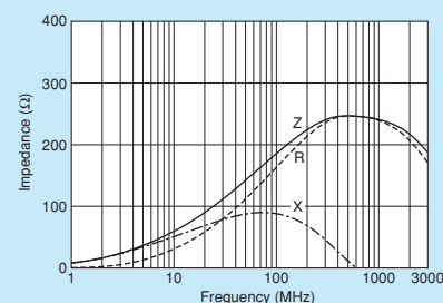
BLM18EG181SH1
