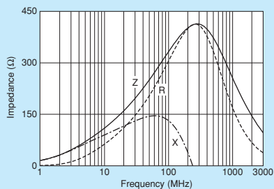
BLM18PG331SZ1/BLM18PG331SH1
