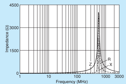
BLM18BA750SZ1/BLM18BA750SH1
