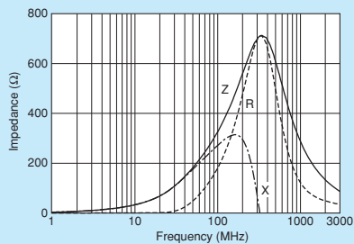
BLM18BD331SZ1/BLM18BD331SH1
