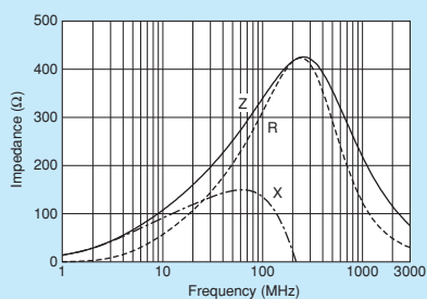
BLM18AG331SZ1/BLM18AG331SH1
