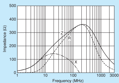
BLM18SG331TZ1
