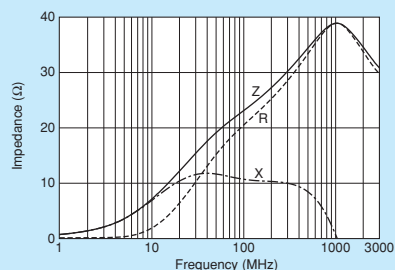
BLM03PG220SZ1
