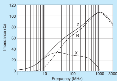
BLM03AG700SZ1
